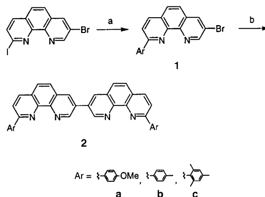
Scheme 2. a) Arylboronic acid, [\text{Pd}(\text{PPh}_3)_4] , \text{Ba}(\text{OH})_2 , 1,2-dimethoxyethane, \text{H}_2\text{O} , reflux; b) \text{NiCl}_2 \cdot 6\text{H}_2\text{O} , \text{PPh}_3 , \text{Zn} , DMF, 50^\circ\text{C} .
